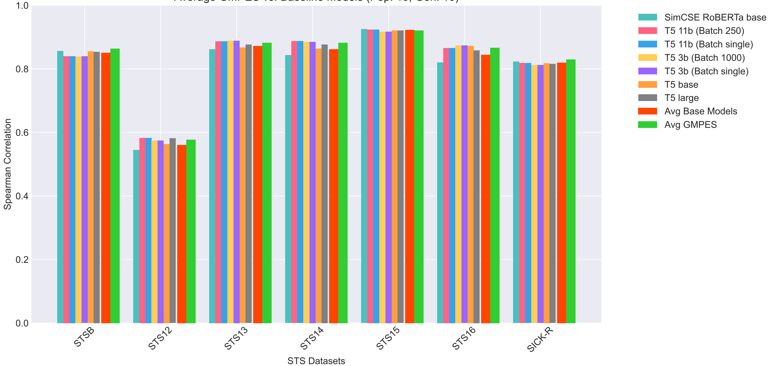
Average GMPES vs. Baseline Models (Pop: 10, Gen: 10)
